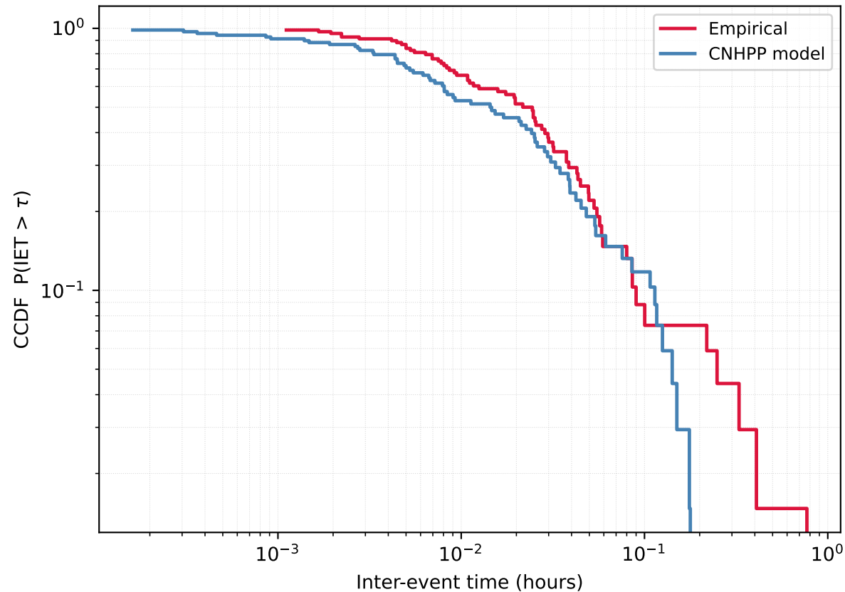
User 1179144696 - Empirical vs CNHPP model
